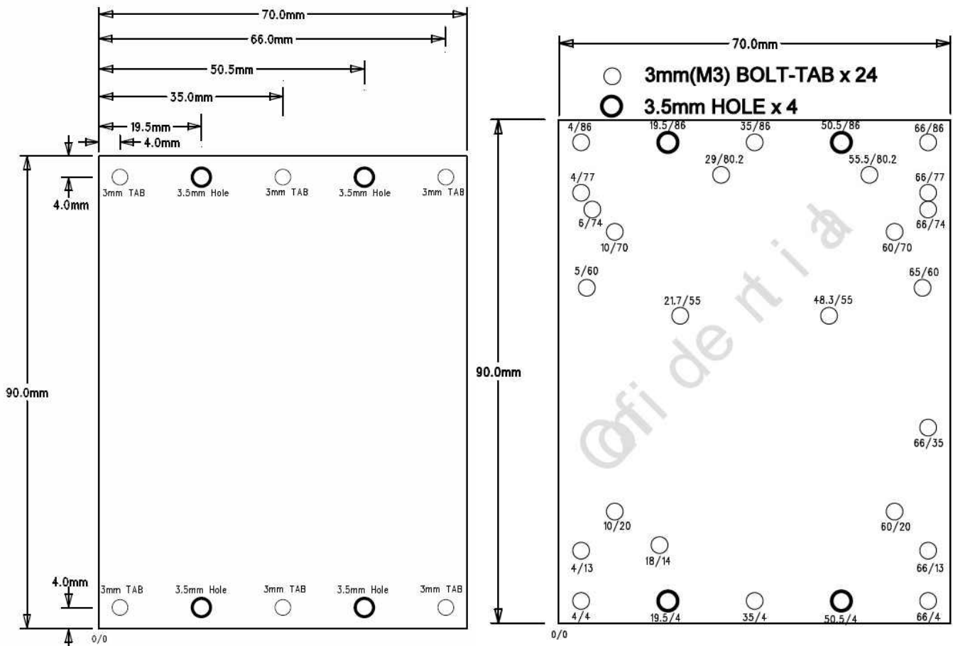
( TOP VIEW )
